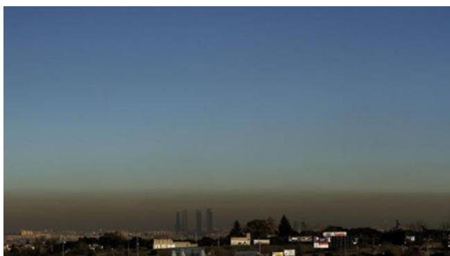
Anticyclonic situation with pollutants contained in the Madrid air mass
